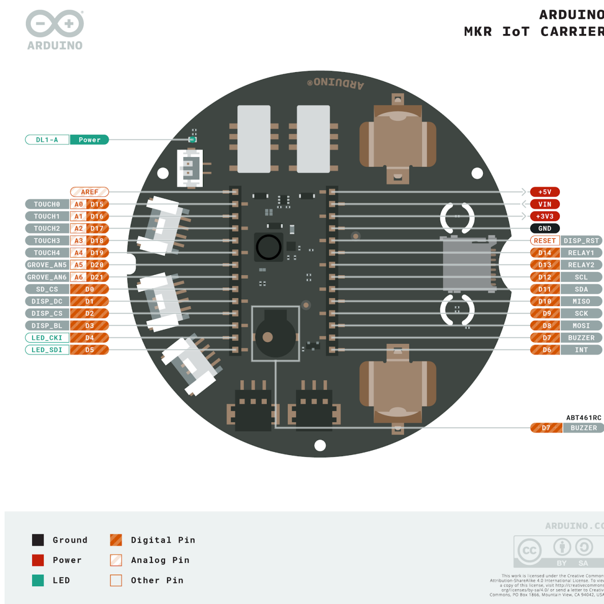
Pinout
